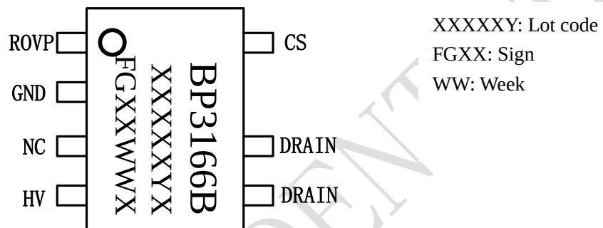
Figure 2. Pin configuration
